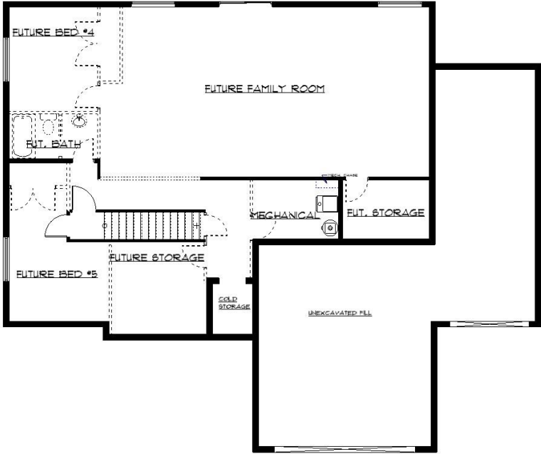
Basement
